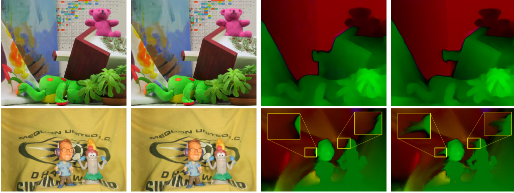
Figure 9: Comparison of results obtained with HSV or RGB colour representation. First row, from left to right: (a) Frame 10 of the Teddy sequence. (b) Frame 11. (c) Result when using the HSV colour space ( AAE = 3.94^\circ ). (d) Same for the RGB colour space ( AAE = 2.64^\circ ). Second row, from left to right: (e) Frame 10 of the Mequon sequence. (f) Frame 11. (g) Result when using the HSV colour space ( AAE = 2.28^\circ ). (h) Same for the RGB colour space ( AAE = 2.84^\circ )
