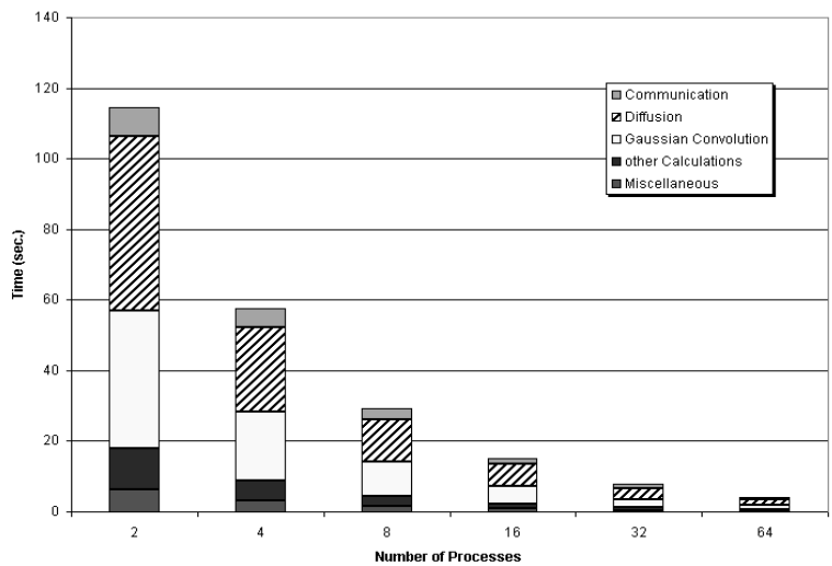
Fig. 6. Myrinet execution time breakdown using slice partitioning
