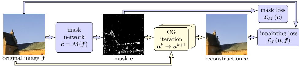
Figure 6.10: Our Mask Optimisation Architecture. The mask network and its losses are coloured in blue, our newly introduced sequence of CG iterations is given in yellow.
